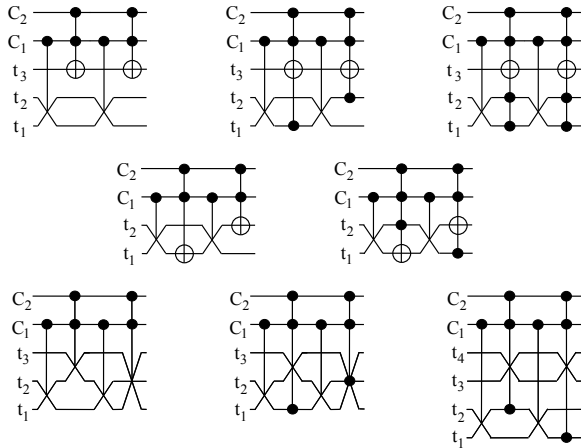
Figure 5: A group of semi passes.
